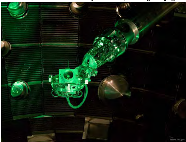
Figure 5-6. NIF's final optics inspection system, when extended into the target chamber from a diagnostic instrument manipulator, can produce images of all 192 beamline final optics assemblies.
