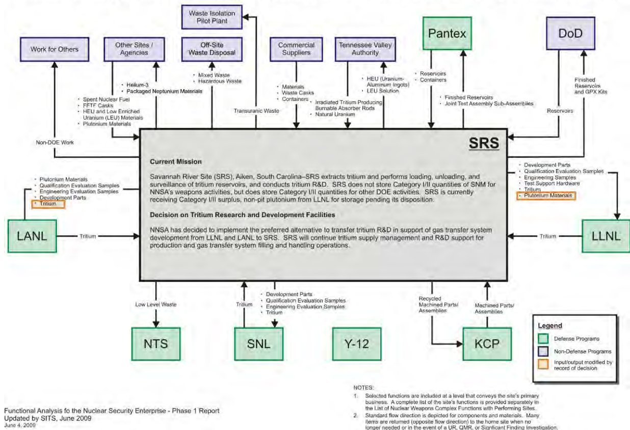
Figure 1-11. Illustrative mission-critical facility external interface diagram for SRS. Example of the process inputs, outputs, and activities that must be integrated at Nuclear Security Enterprise locations
